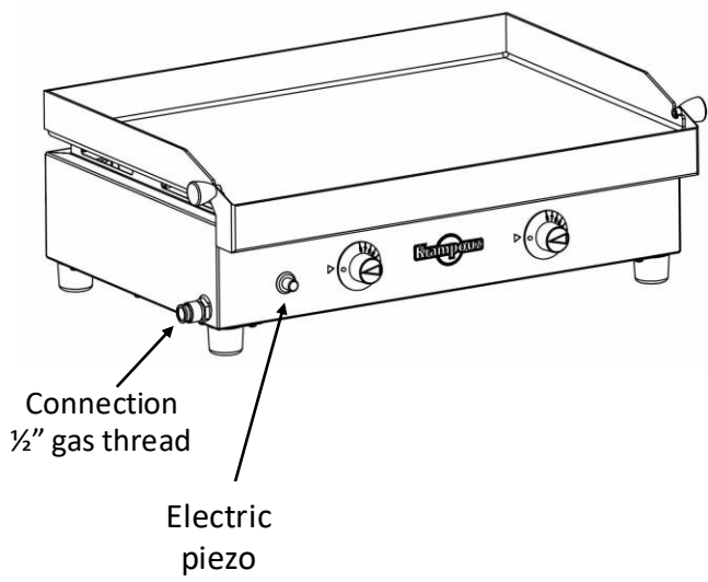
FIGURE 2 – CONNECTION
